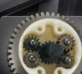
Planetary Differential
